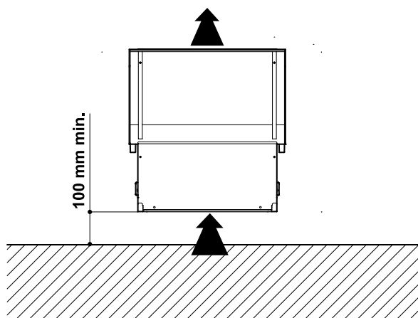
VERTICAL INSTALLATION
