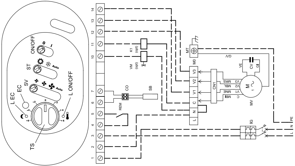
WALL-MOUNTED VERSION
